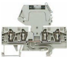
Disconnect terminals diode or fuse carrier
