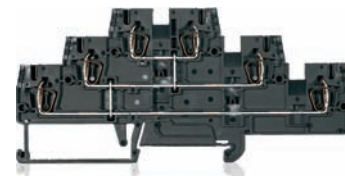
Double deck terminals vertical connection (with common points)
